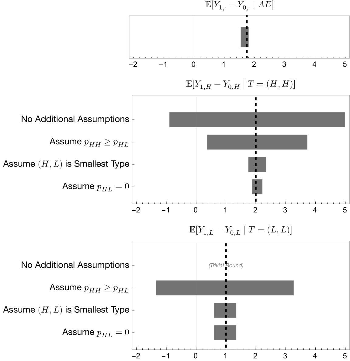
FIGURE 6. Results of Design 2. The dashed black line represents the true value of the parameter.
