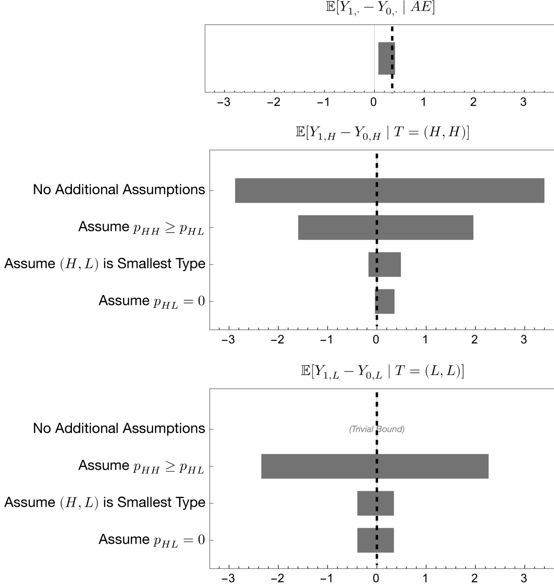
FIGURE 5. Results for design 1. The dashed black line represents the true value of the parameter.
